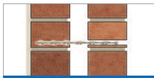
6 Replacing cavity wall ties
