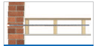
4 Stabilising bowed walls into joist sides
