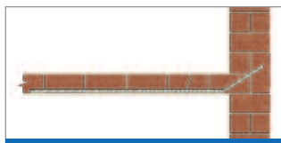
5 Reconnecting internal walls with external walls
